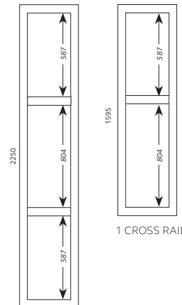
2 CROSS RAILS
